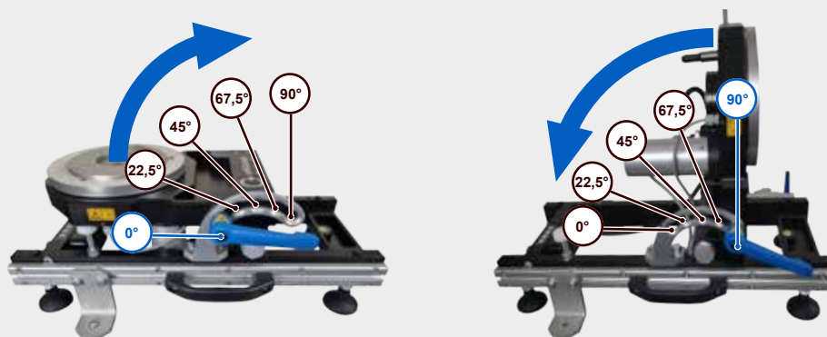
Swivel plate adjustable in 5 positions (0-90°).
